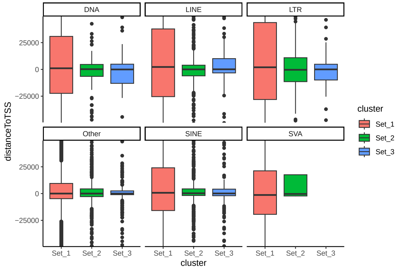
Distance to TSS by class in H3K9me3 of overlapping ROIs
